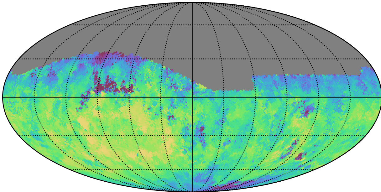
noroll_mjdp120_v3.4_10yrs Yr 1 z band: Median fiveSigmaDepth
