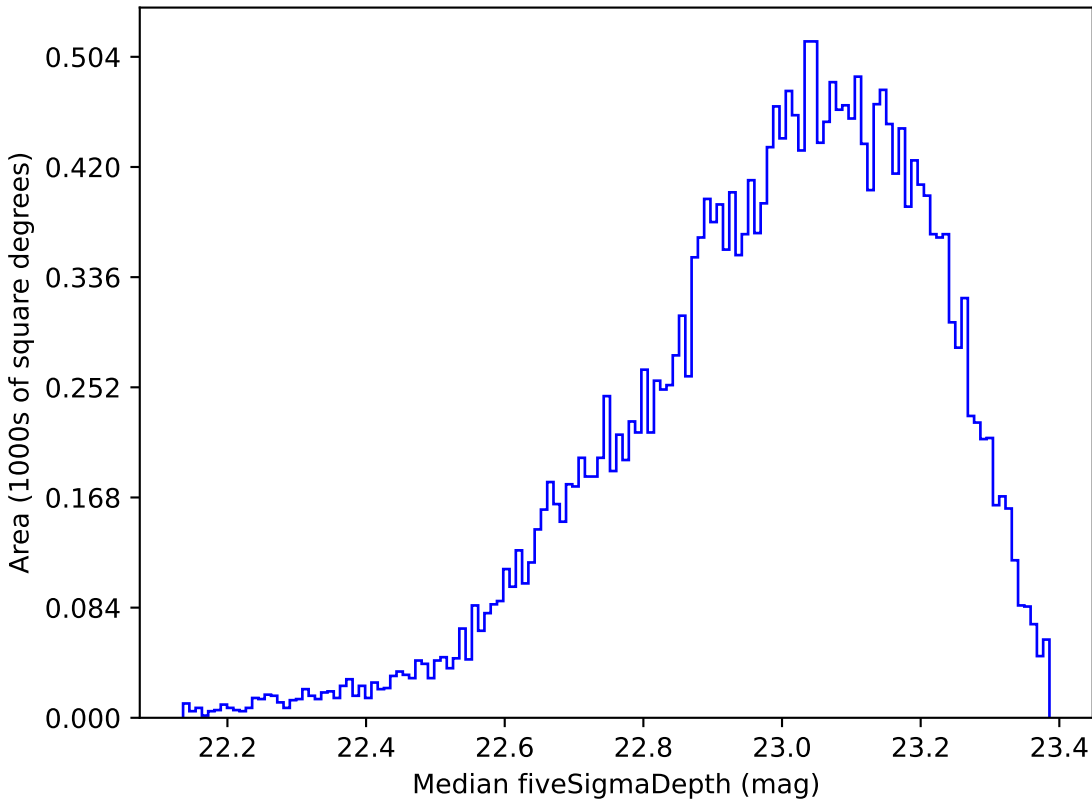
noroll_mjdp120_v3.4_10yrs Yr 1 z band: Median fiveSigmaDepth
