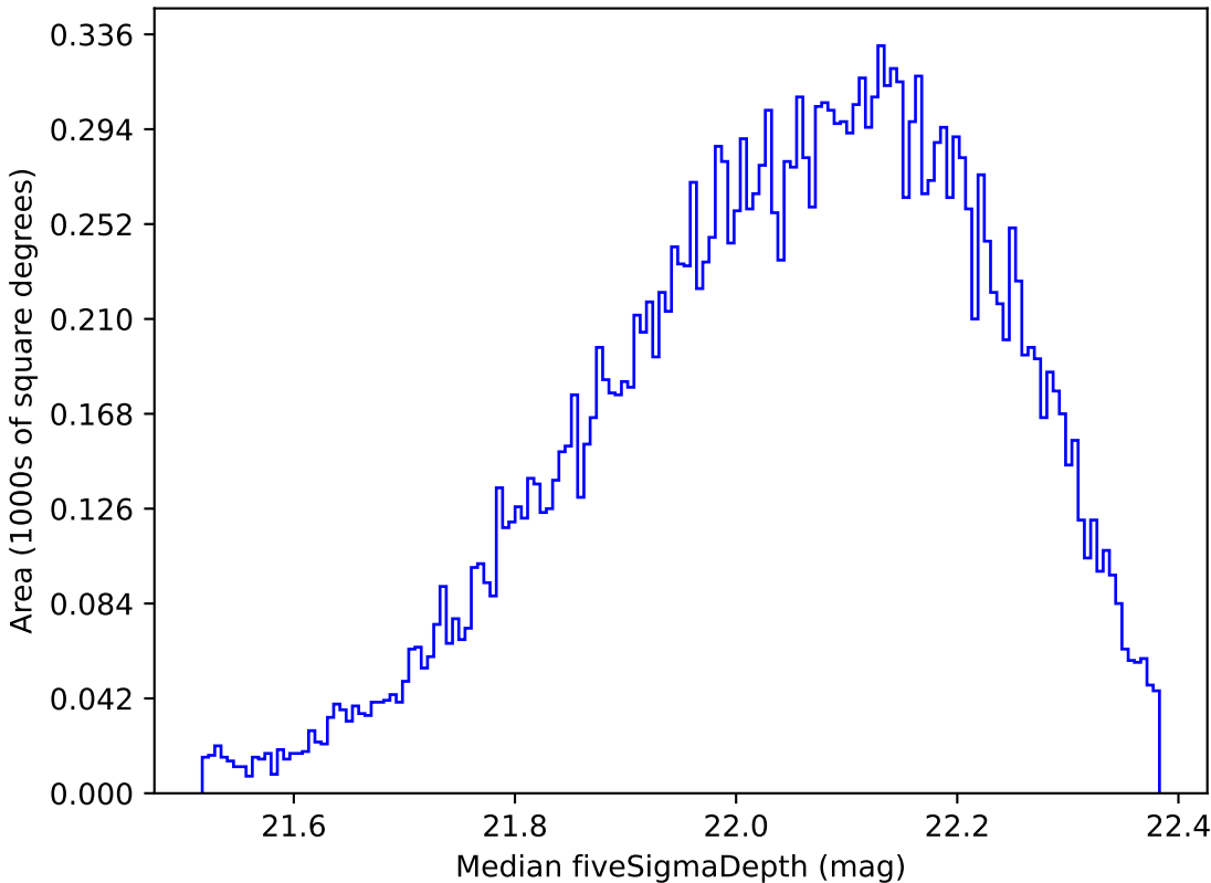
noroll_mjdp120_v3.4_10yrs Yr 1 y band: Median fiveSigmaDepth
