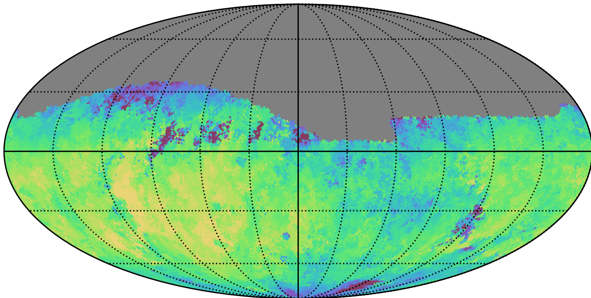
noroll_mjdp120_v3.4_10yrs Yr 1 r band: Median fiveSigmaDepth
