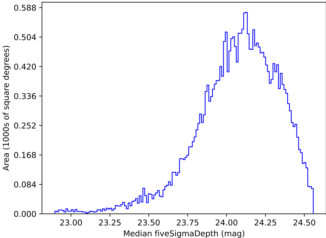
noroll_mjdp120_v3.4_10yrs Yr 1 r band: Median fiveSigmaDepth
