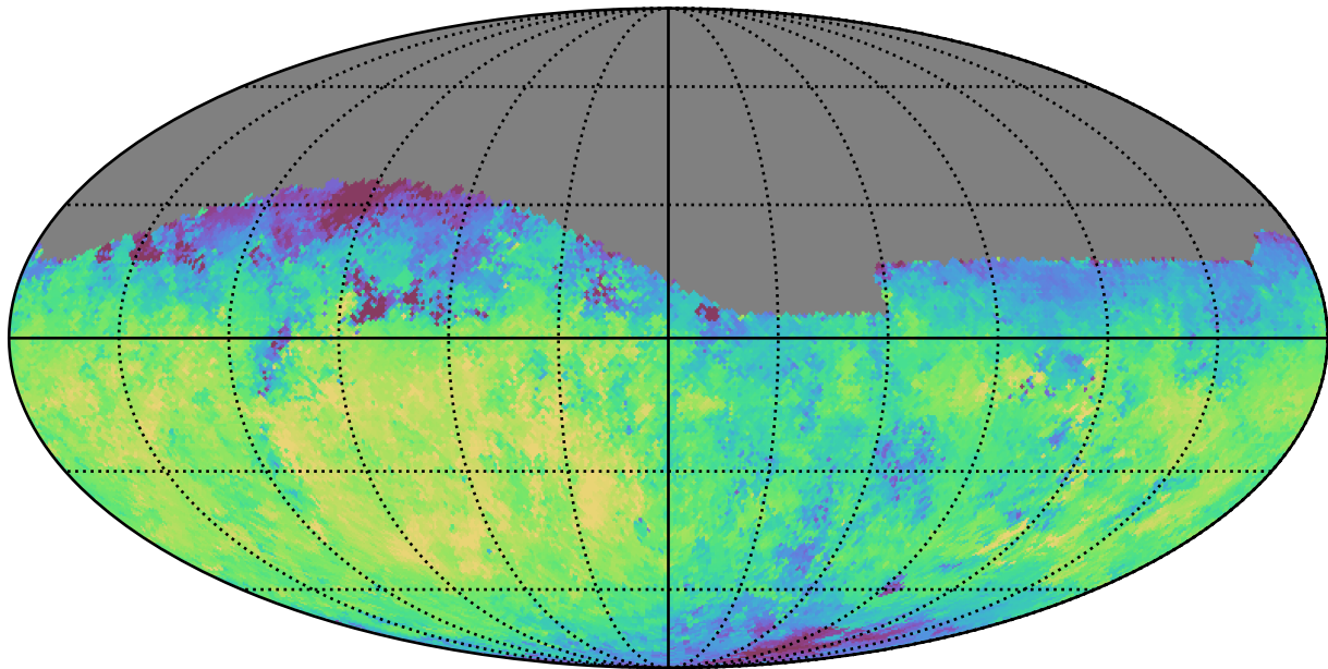
noroll_mjdp120_v3.4_10yrs Yr 1 i band: Median fiveSigmaDepth
