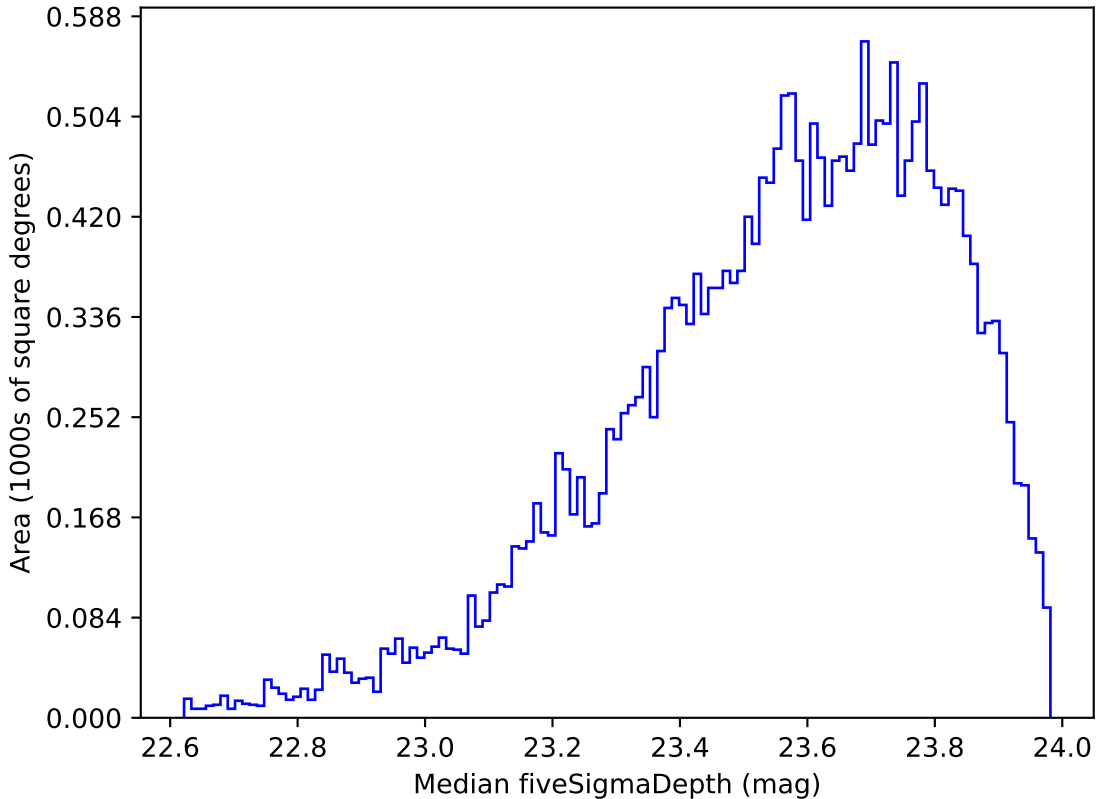
noroll_mjdp120_v3.4_10yrs Yr 1 i band: Median fiveSigmaDepth
