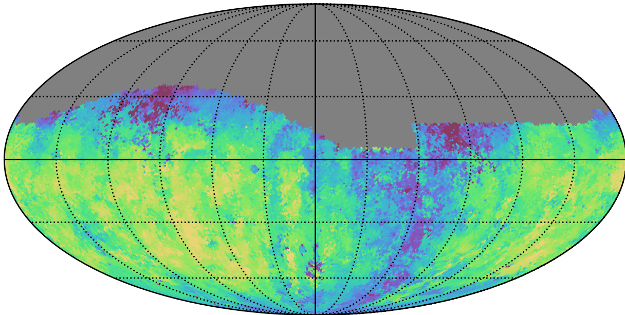
noroll_mjdp120_v3.4_10yrs Yr 1 g band: Median fiveSigmaDepth
