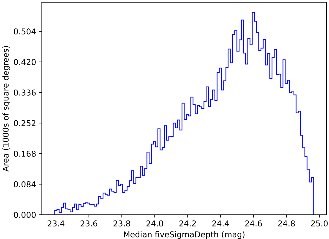
noroll_mjdp120_v3.4_10yrs Yr 1 g band: Median fiveSigmaDepth
