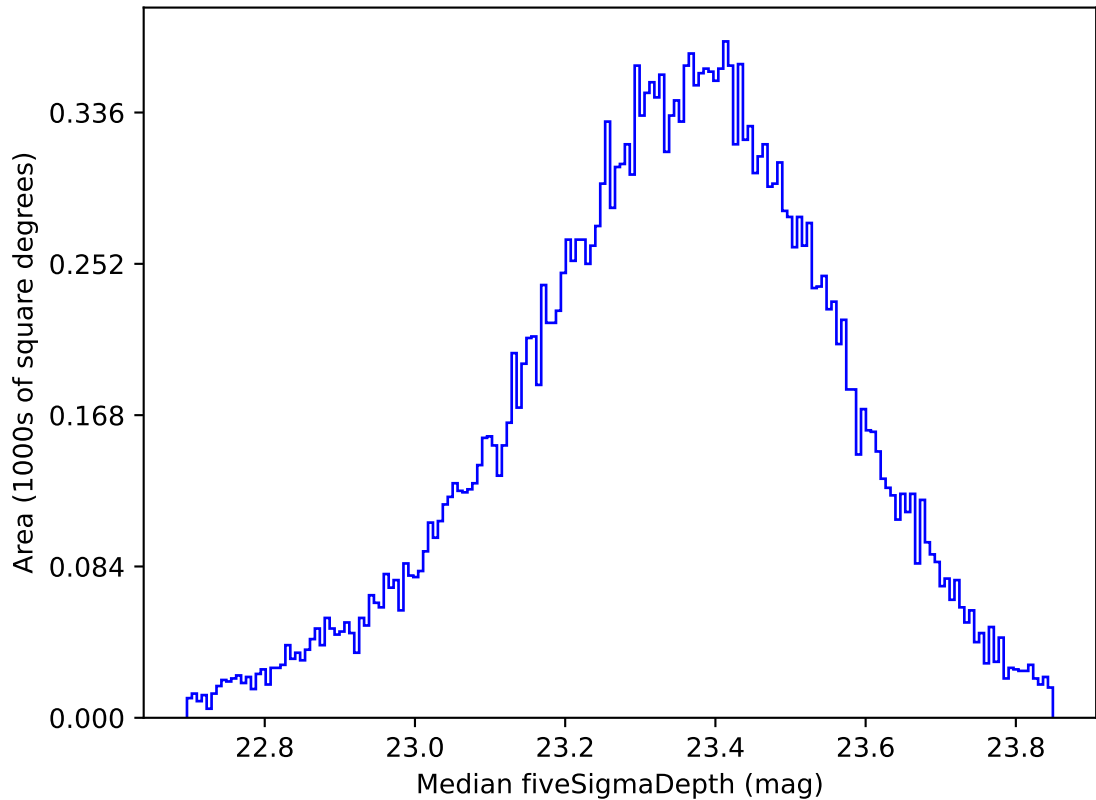
noroll_mjdp120_v3.4_10yrs Yr 1 all bands: Median fiveSigmaDepth
