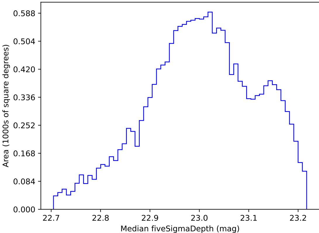
noroll_mjdp120_v3.4_10yrs WFD z band: Median fiveSigmaDepth
