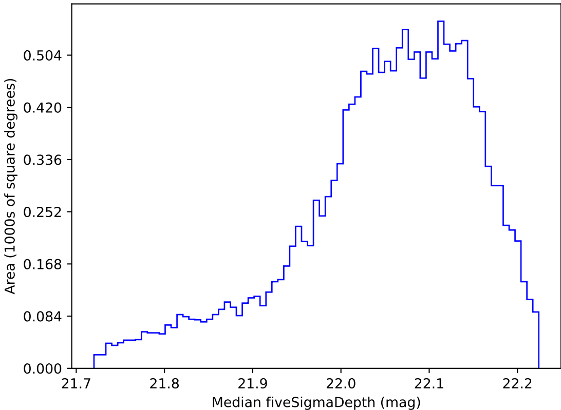
noroll_mjdp120_v3.4_10yrs WFD y band: Median fiveSigmaDepth
