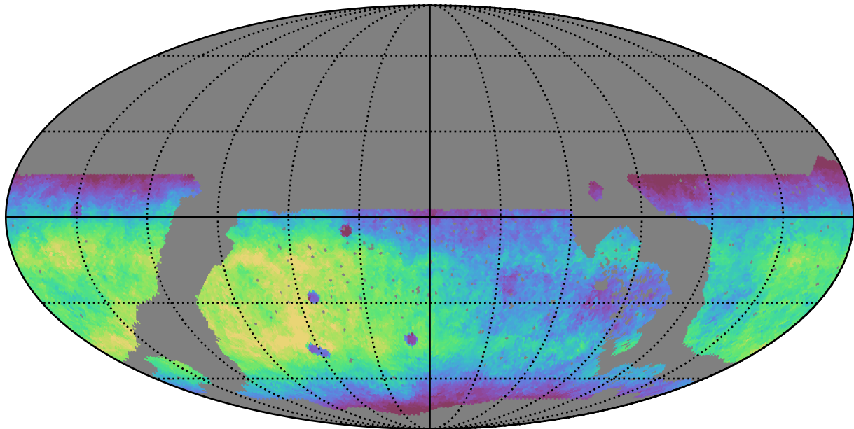
noroll_mjdp120_v3.4_10yrs WFD r band: Median fiveSigmaDepth
