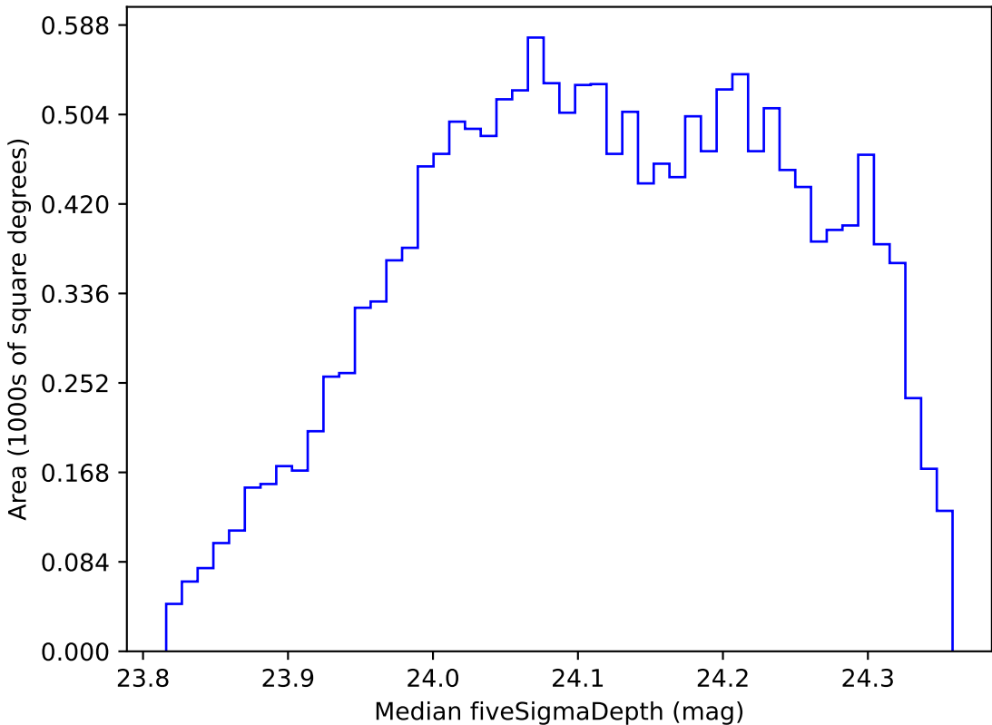
noroll_mjdp120_v3.4_10yrs WFD r band: Median fiveSigmaDepth
