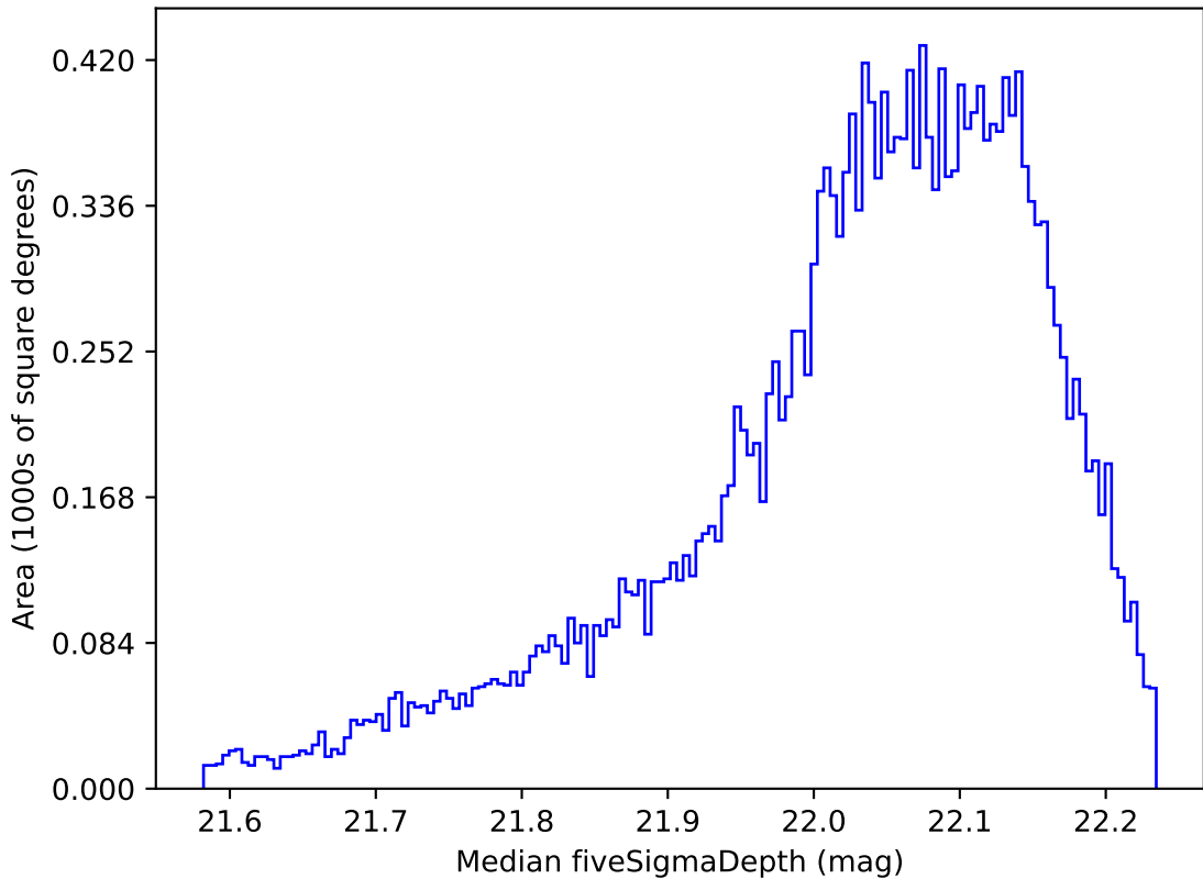
noroll_mjdp120_v3.4_10yrs All sky y band: Median fiveSigmaDepth
