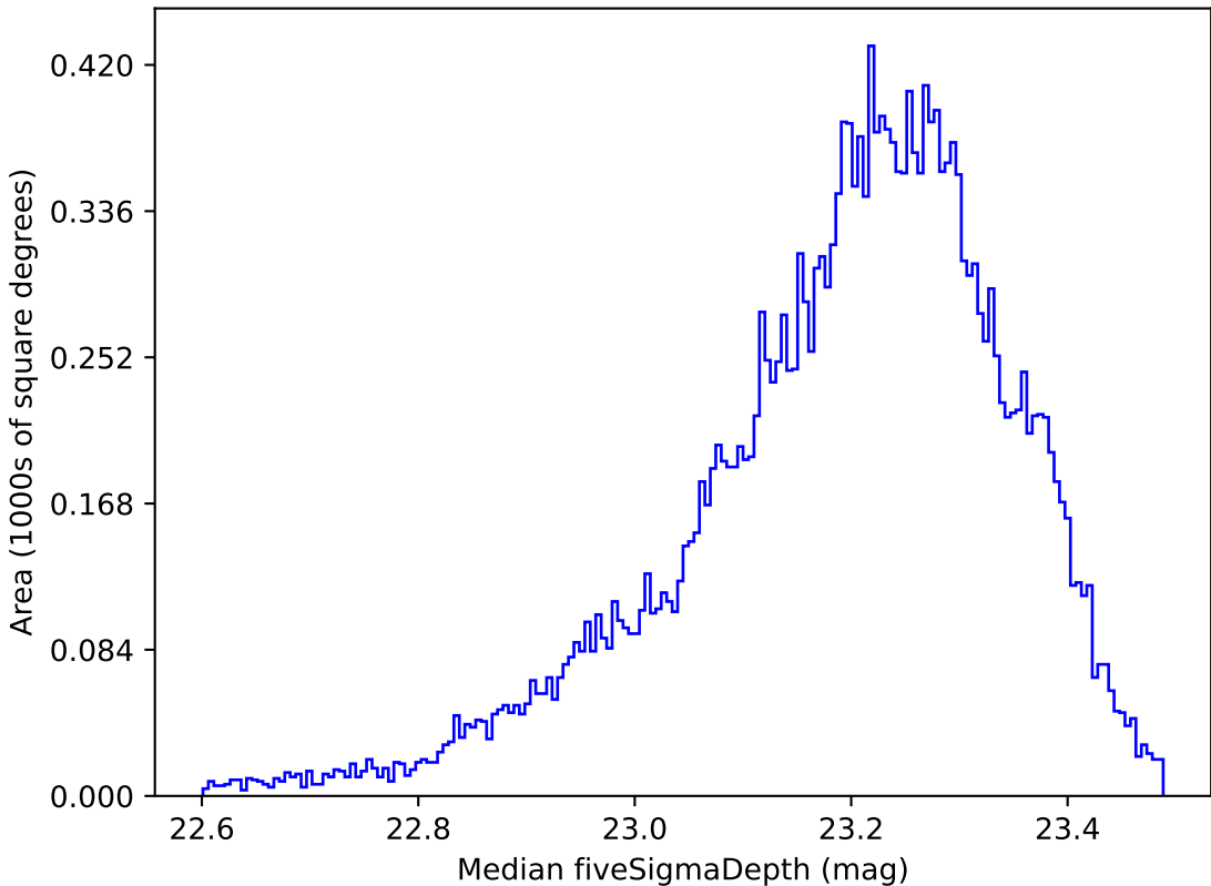
noroll_mjdp120_v3.4_10yrs All sky u band: Median fiveSigmaDepth
