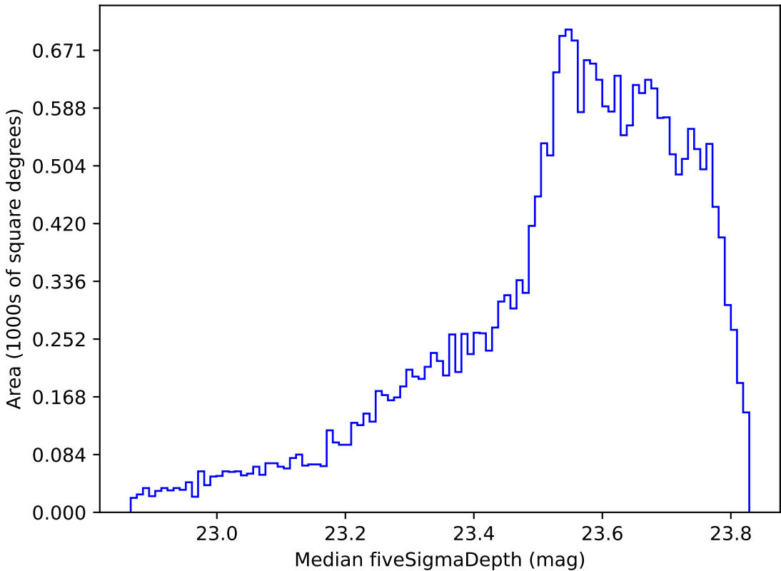
noroll_mjdp120_v3.4_10yrs All sky i band: Median fiveSigmaDepth
