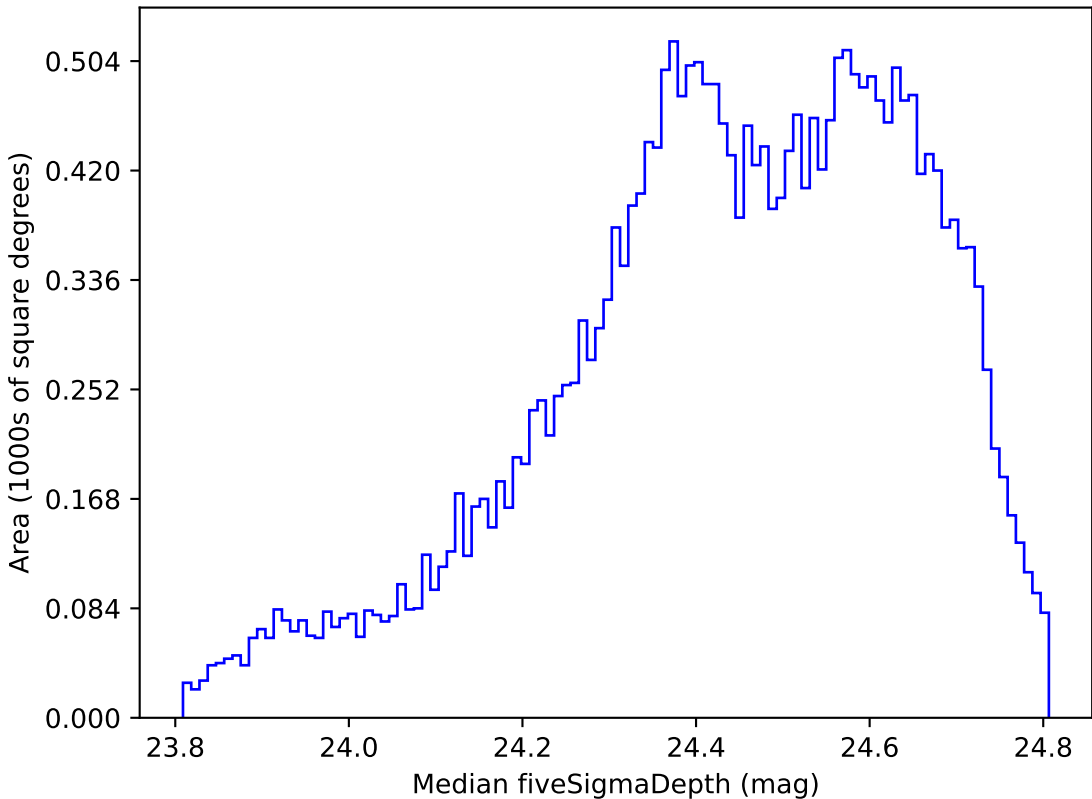
noroll_mjdp120_v3.4_10yrs All sky g band: Median fiveSigmaDepth
