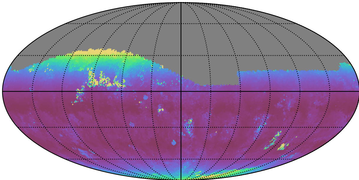
noroll_mjdp120_v3.4_10yrs Yr 1 z band: Median airmass
