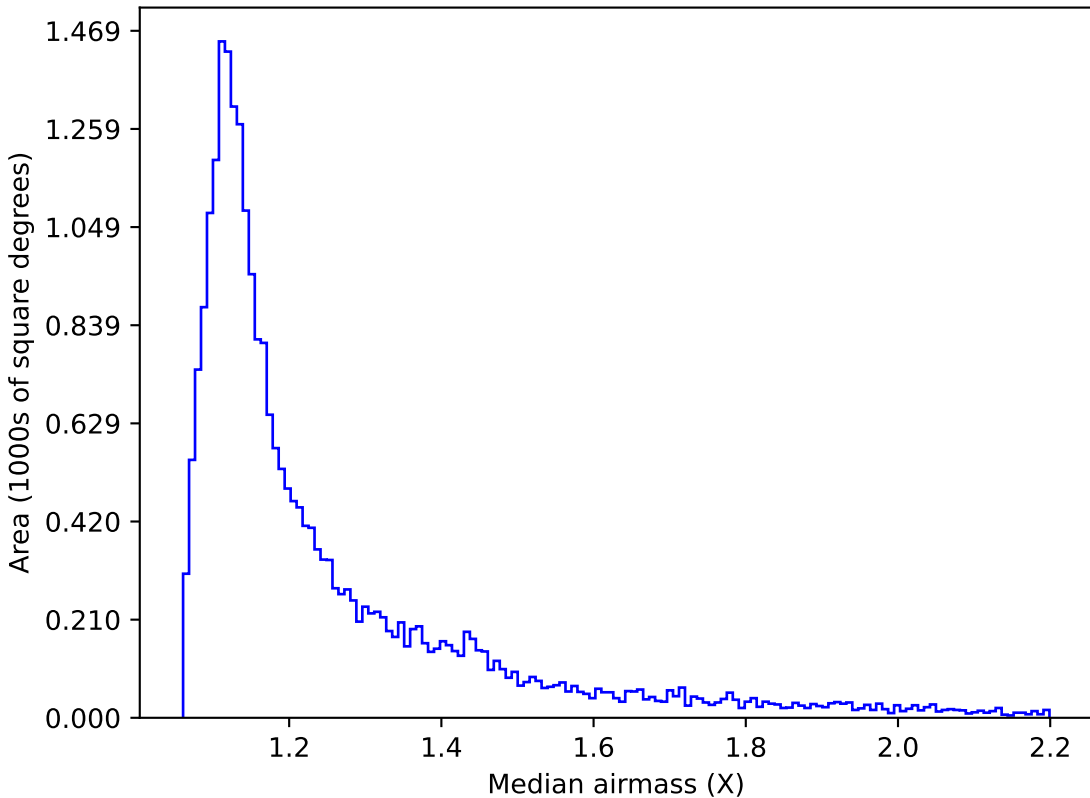
noroll_mjdp120_v3.4_10yrs Yr 1 z band: Median airmass
