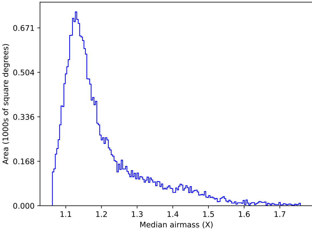
noroll_mjdp120_v3.4_10yrs Yr 1 y band: Median airmass
