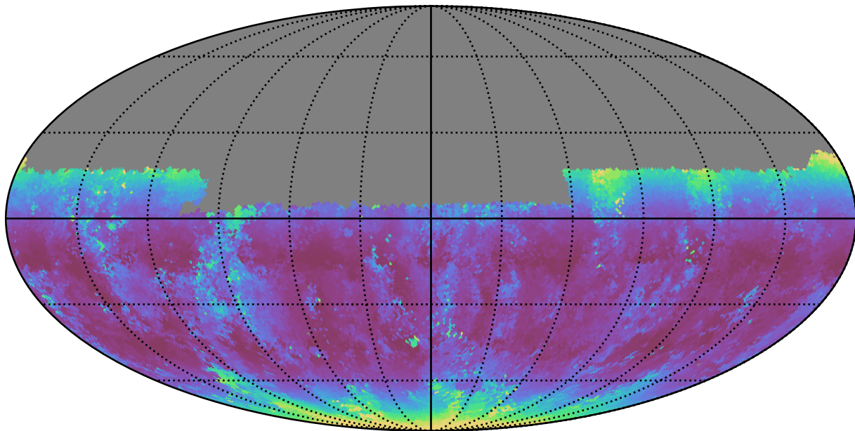
noroll_mjdp120_v3.4_10yrs Yr 1 u band: Median airmass
