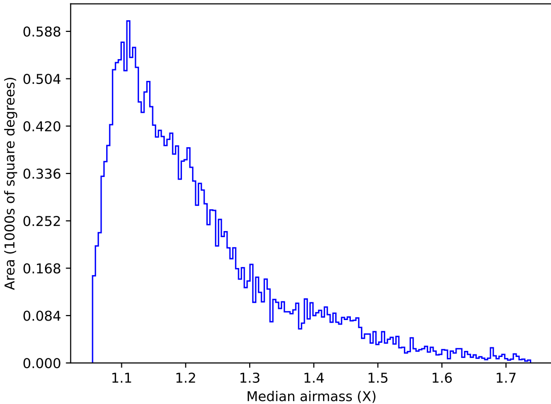
noroll_mjdp120_v3.4_10yrs Yr 1 u band: Median airmass
