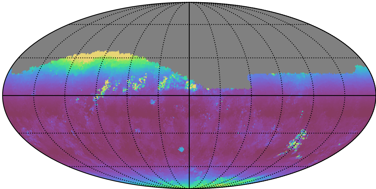
noroll_mjdp120_v3.4_10yrs Yr 1 r band: Median airmass
