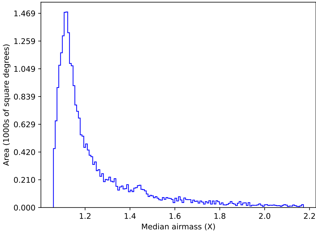
noroll_mjdp120_v3.4_10yrs Yr 1 r band: Median airmass
