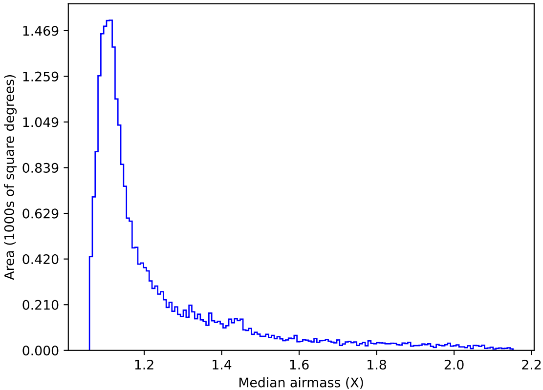
noroll_mjdp120_v3.4_10yrs Yr 1 i band: Median airmass
