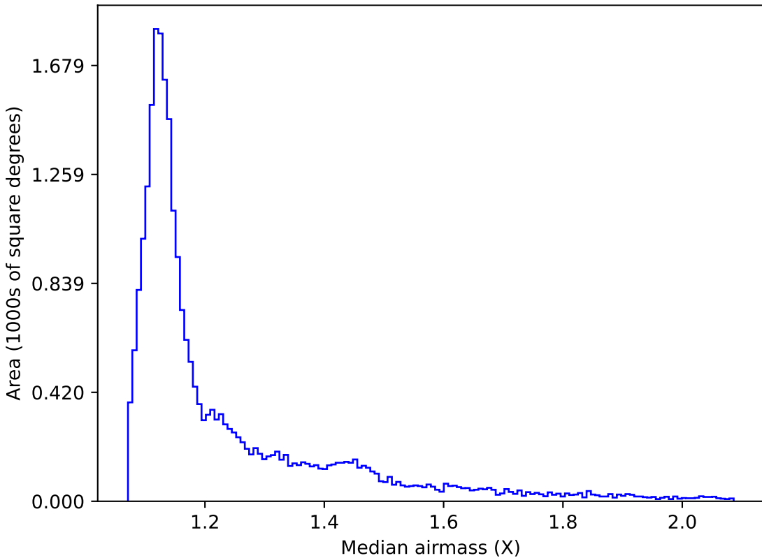
noroll_mjdp120_v3.4_10yrs Yr 1 all bands: Median airmass
