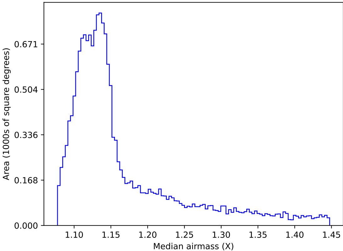
noroll_mjdp120_v3.4_10yrs WFD z band: Median airmass
