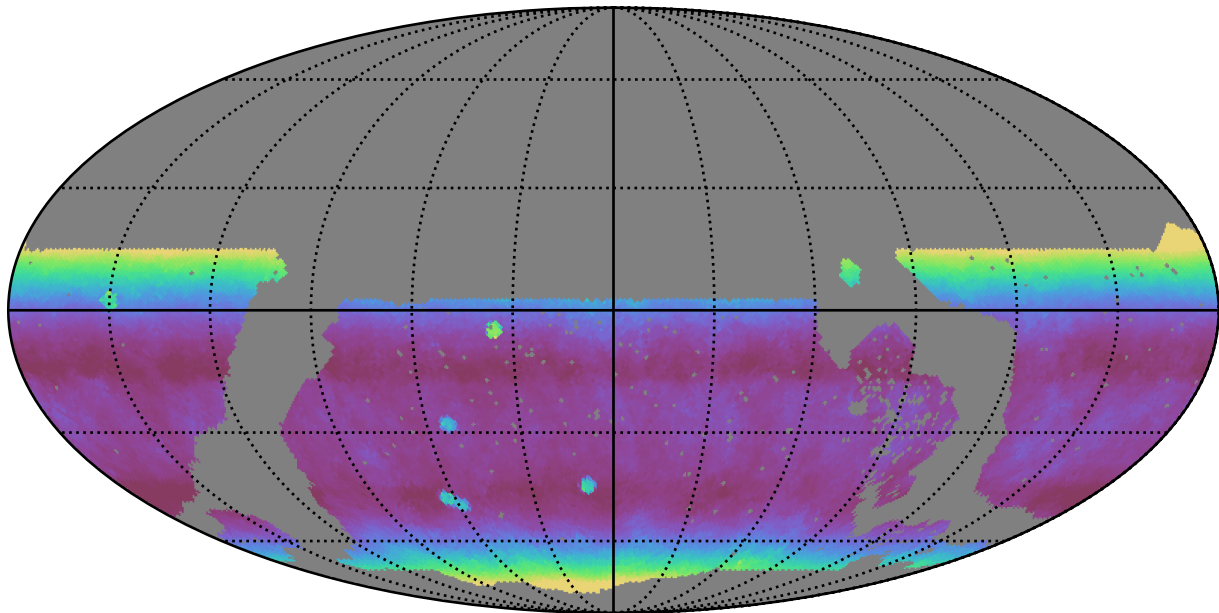
noroll_mjdp120_v3.4_10yrs WFD y band: Median airmass
