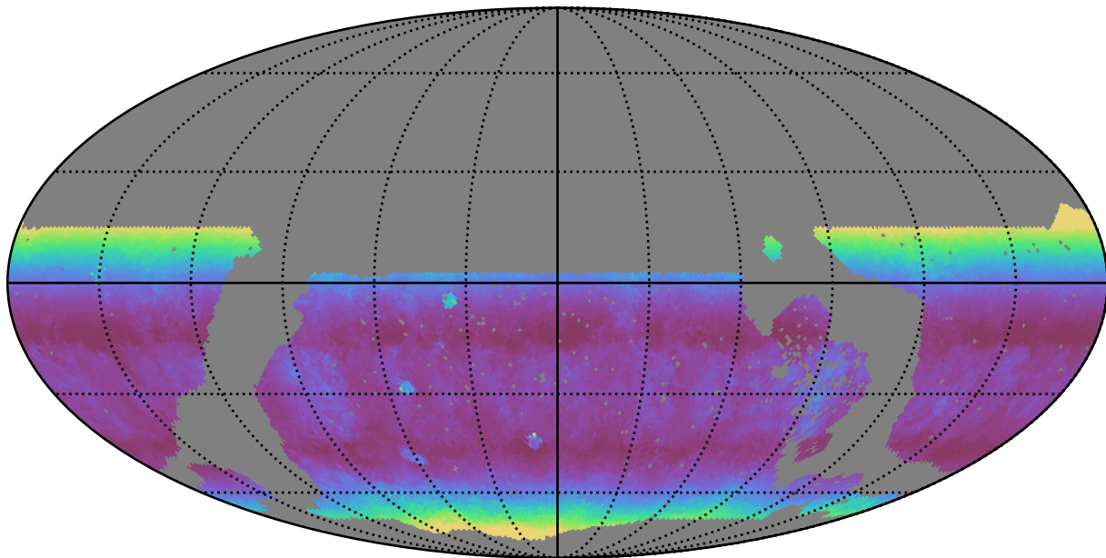
noroll_mjdp120_v3.4_10yrs WFD u band: Median airmass
