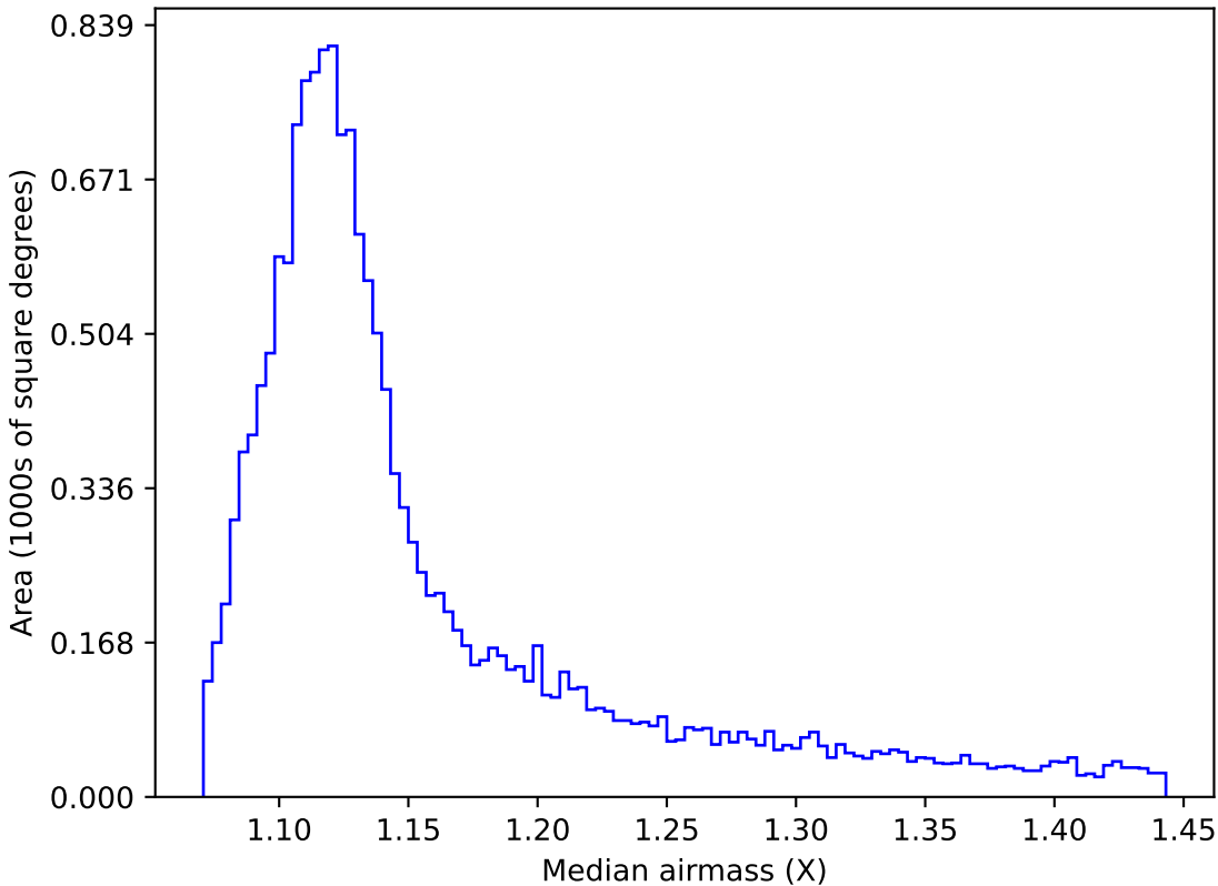
noroll_mjdp120_v3.4_10yrs WFD u band: Median airmass
