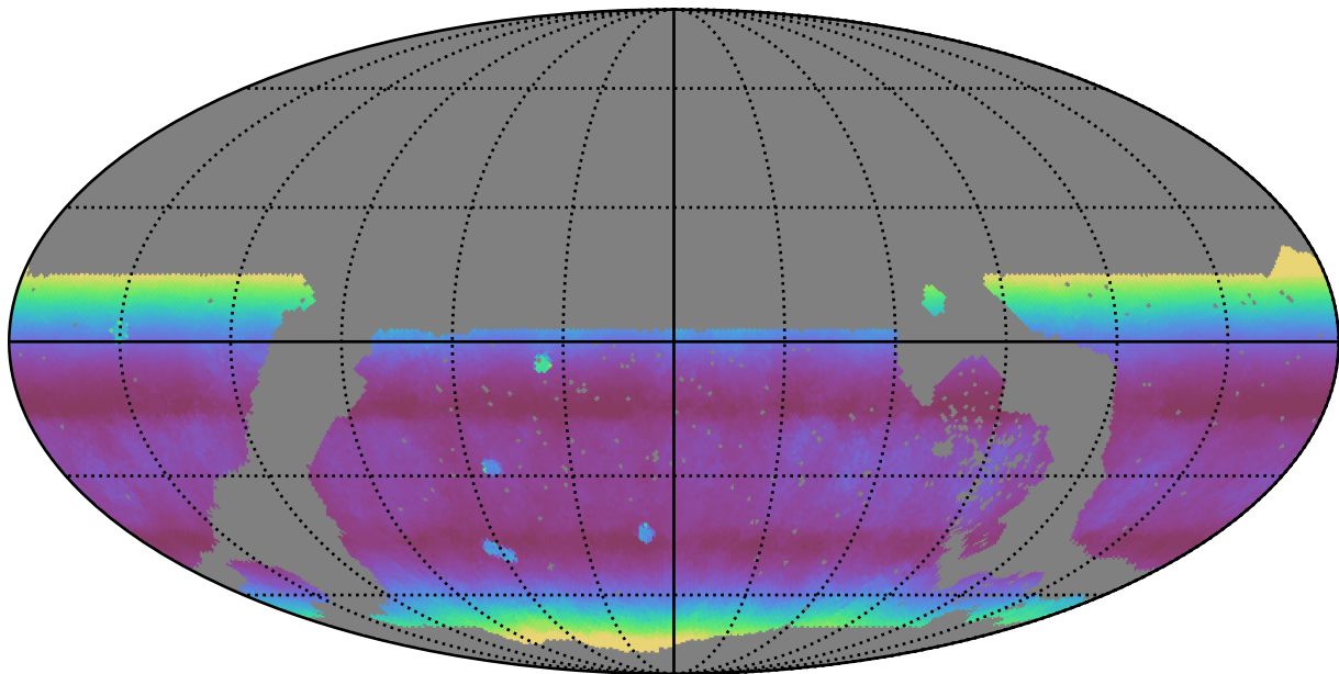
noroll_mjdp120_v3.4_10yrs WFD r band: Median airmass
