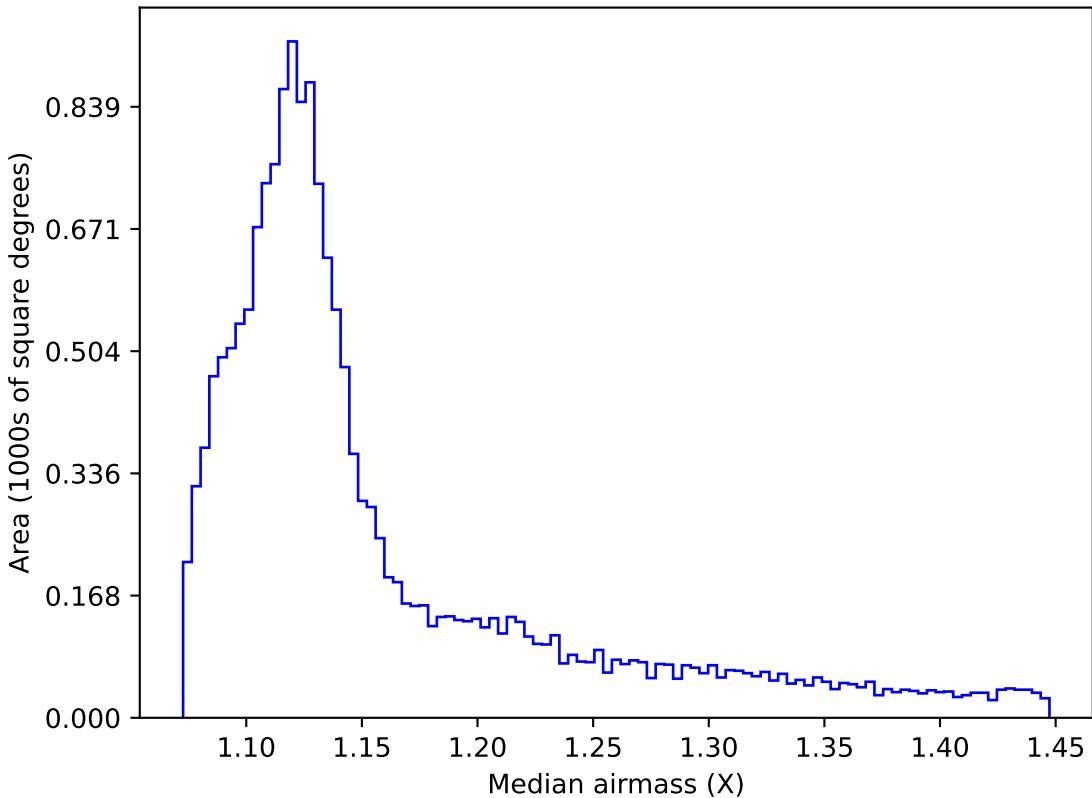
noroll_mjdp120_v3.4_10yrs WFD r band: Median airmass
