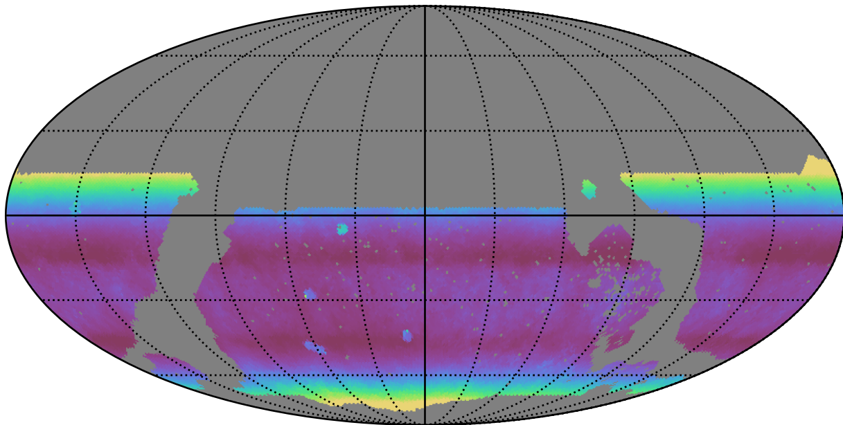
noroll_mjdp120_v3.4_10yrs WFD i band: Median airmass
