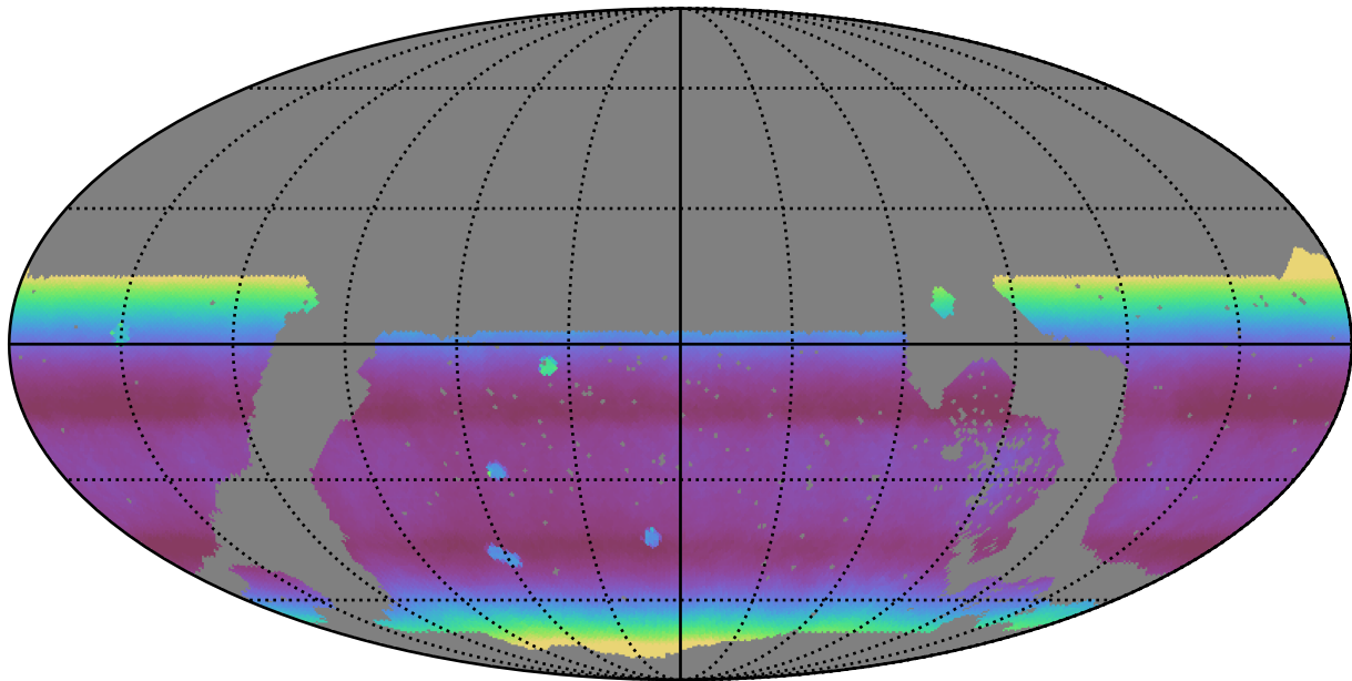
noroll_mjdp120_v3.4_10yrs WFD all bands: Median airmass
