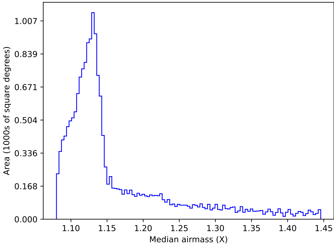
noroll_mjdp120_v3.4_10yrs WFD all bands: Median airmass
