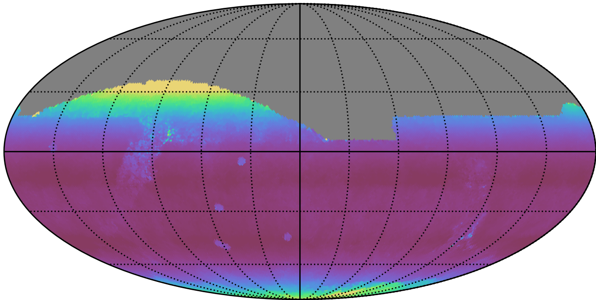
noroll_mjdp120_v3.4_10yrs All sky z band: Median airmass
