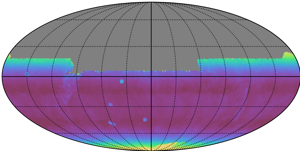
noroll_mjdp120_v3.4_10yrs All sky y band: Median airmass
