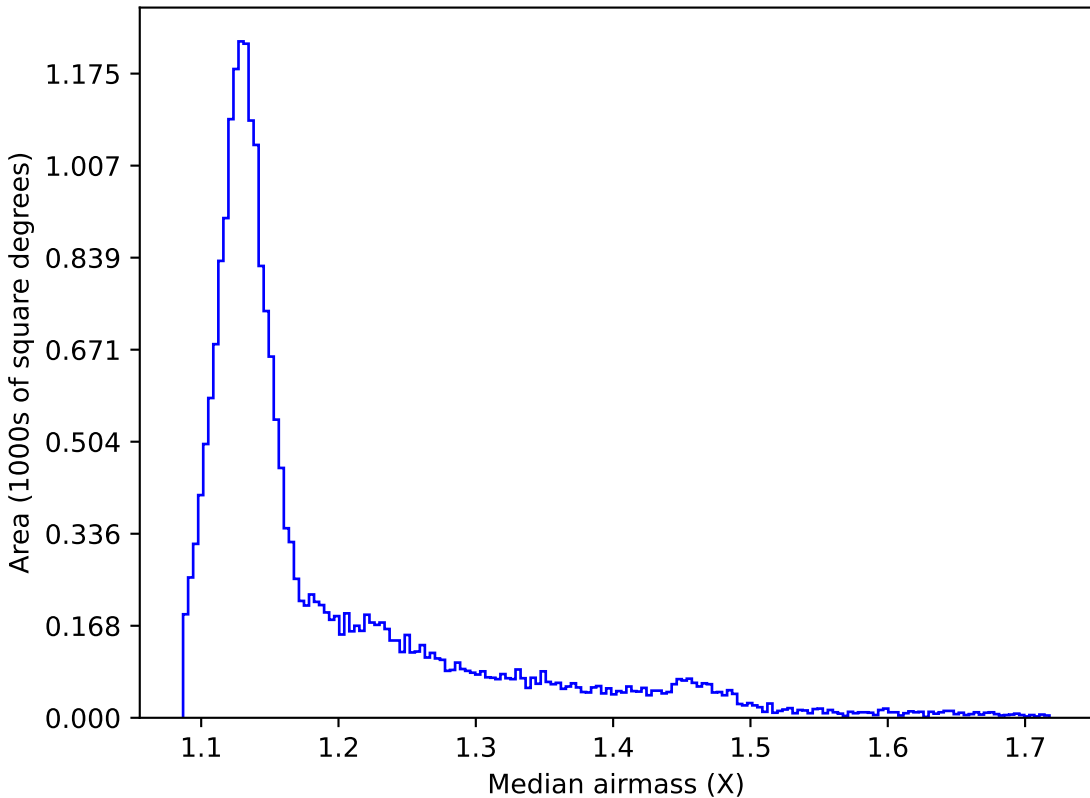
noroll_mjdp120_v3.4_10yrs All sky y band: Median airmass
