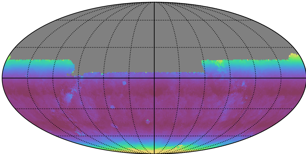
noroll_mjdp120_v3.4_10yrs All sky u band: Median airmass
