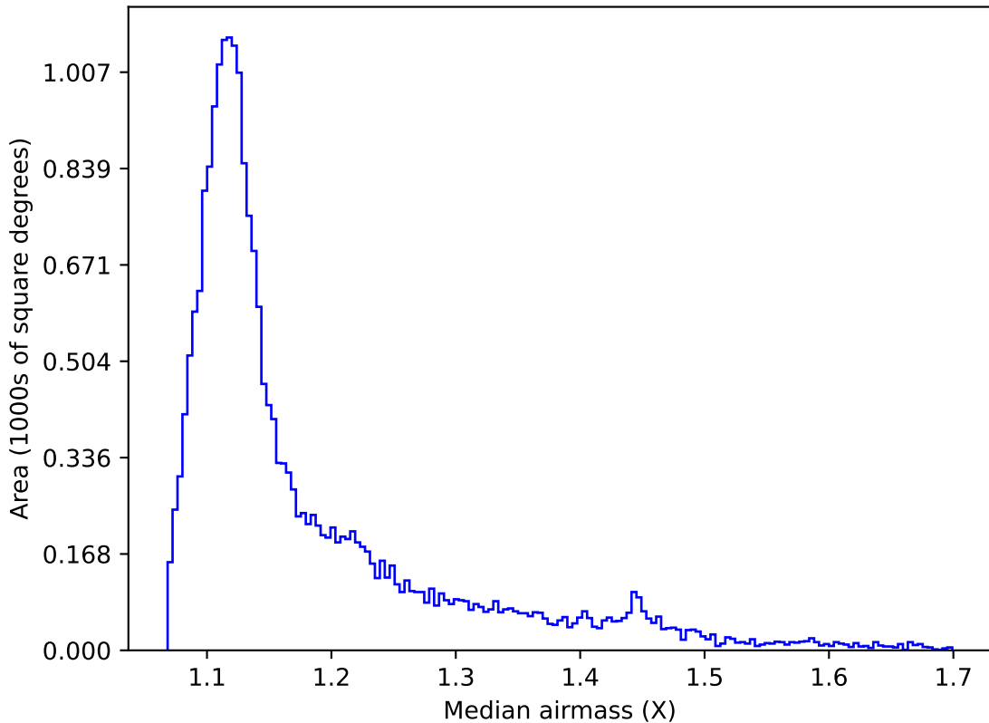
noroll_mjdp120_v3.4_10yrs All sky u band: Median airmass
