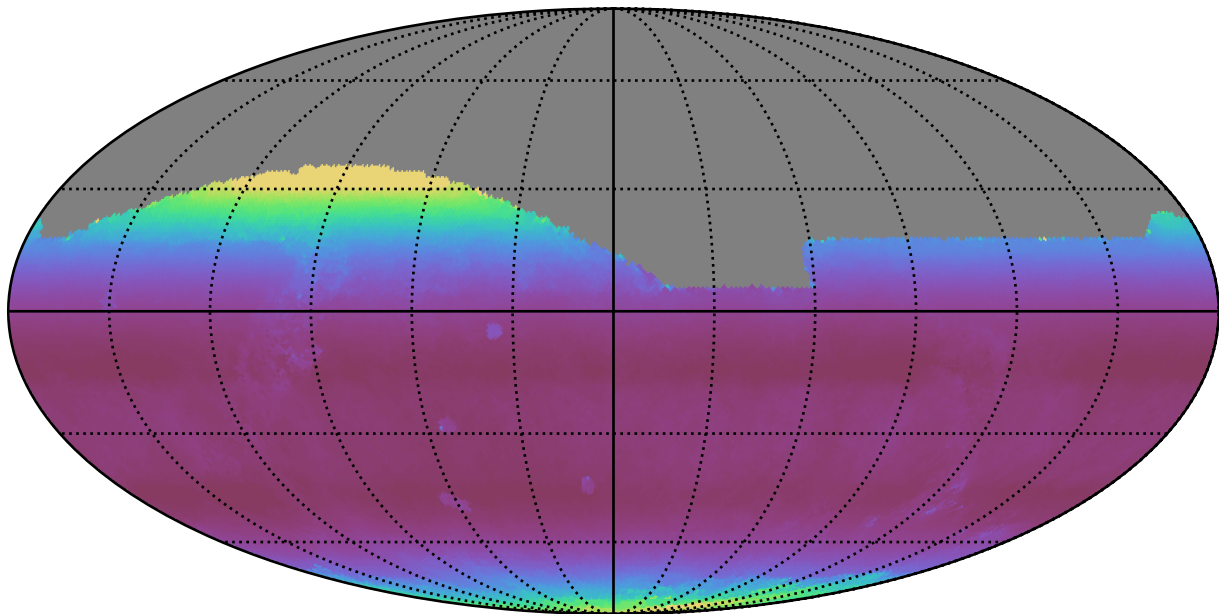
noroll_mjdp120_v3.4_10yrs All sky i band: Median airmass
