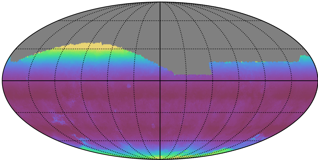
noroll_mjdp120_v3.4_10yrs All sky g band: Median airmass
