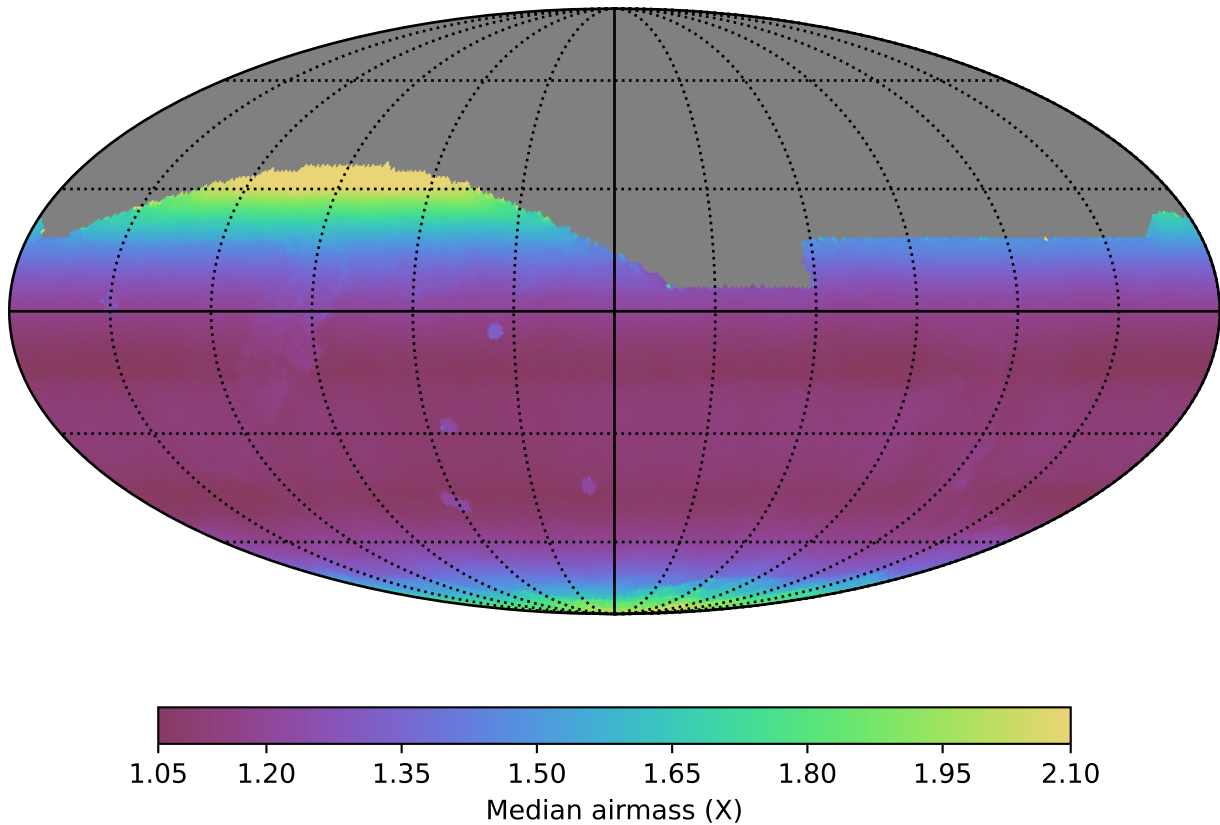
noroll_mjdp120_v3.4_10yrs All sky all bands: Median airmass
