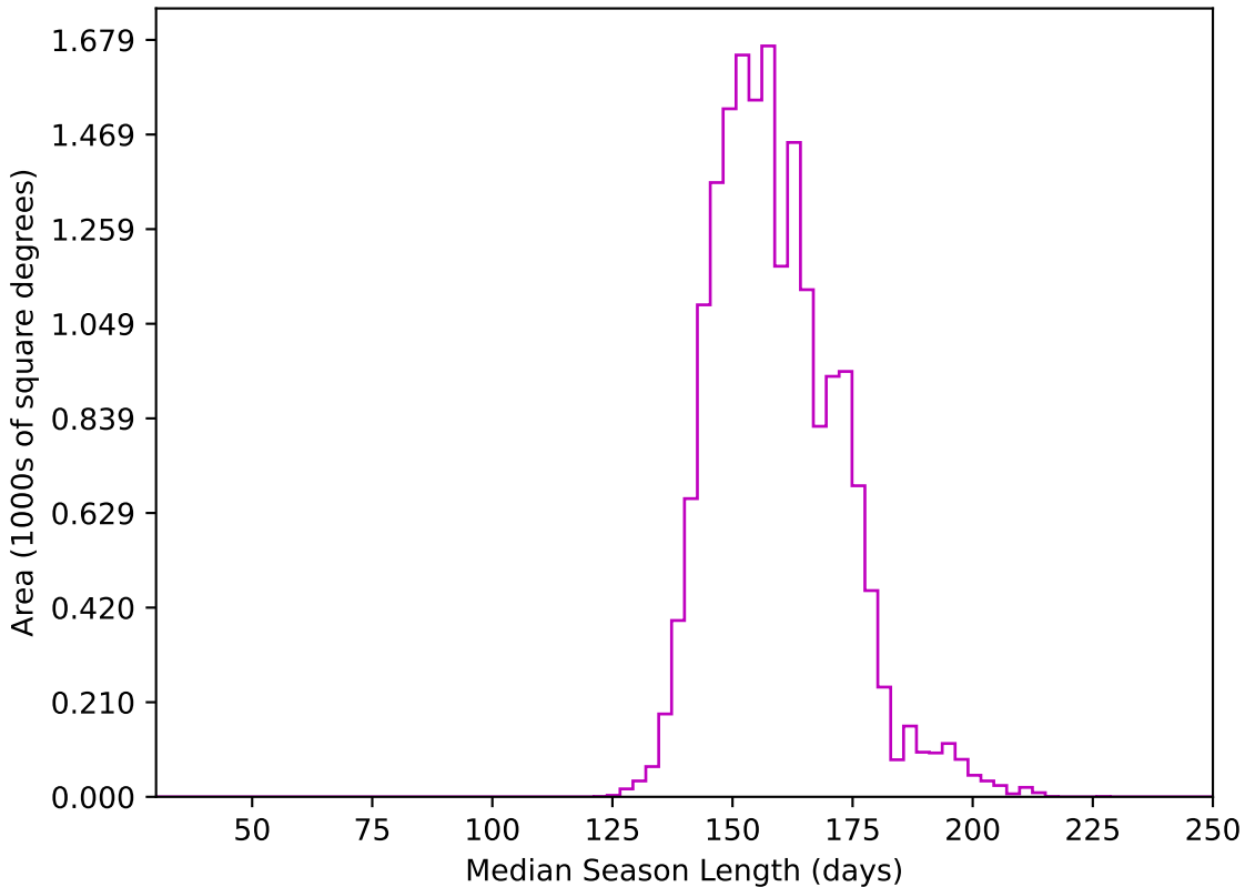
noroll_mjdp120_v3.4_10yrs WFD z band: Median Season Length
