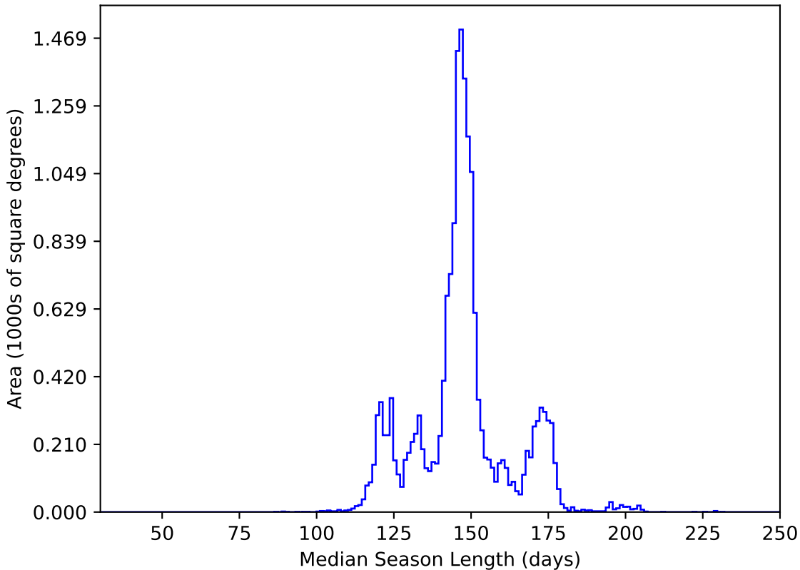
noroll_mjdp120_v3.4_10yrs WFD y band: Median Season Length
