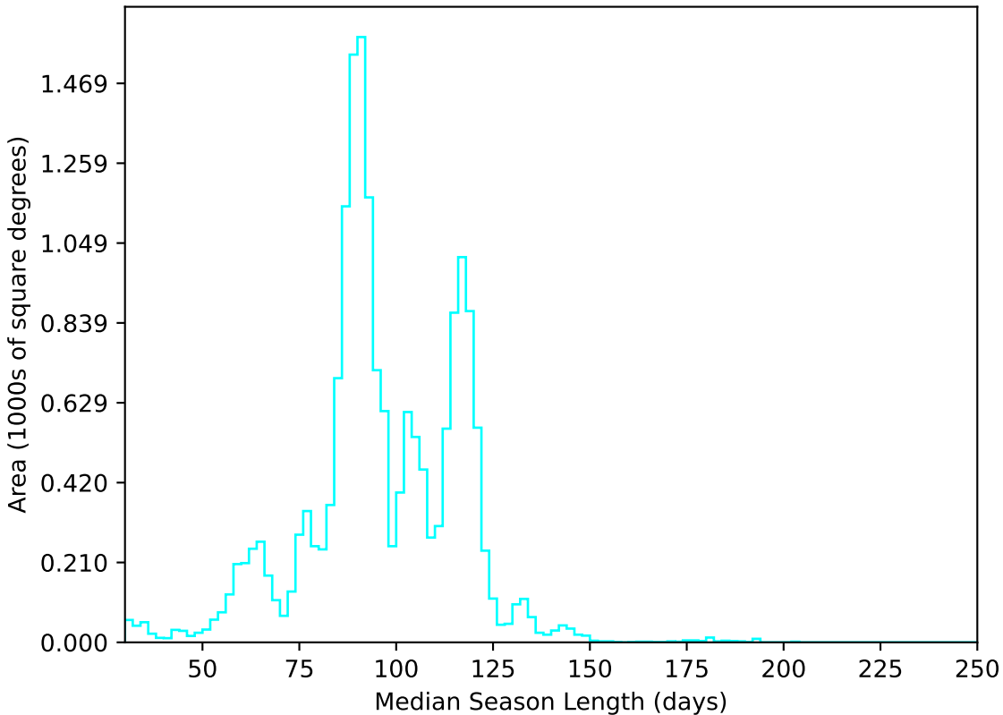
noroll_mjdp120_v3.4_10yrs WFD u band: Median Season Length
