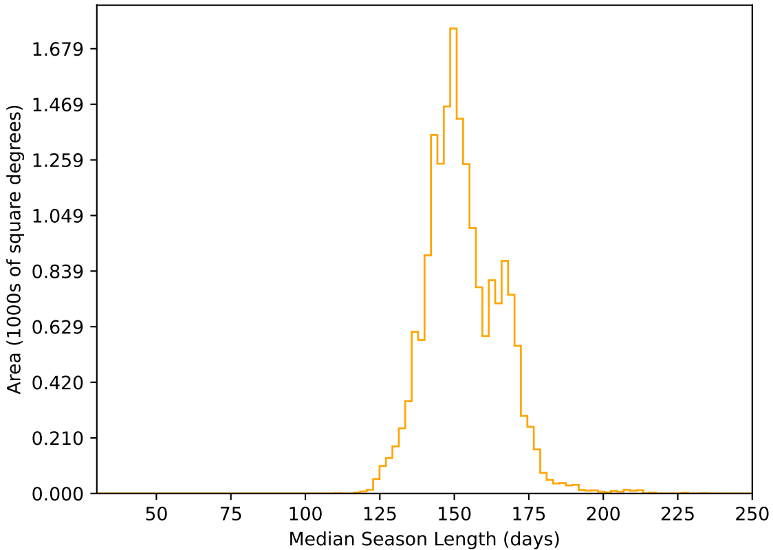
noroll_mjdp120_v3.4_10yrs WFD r band: Median Season Length
