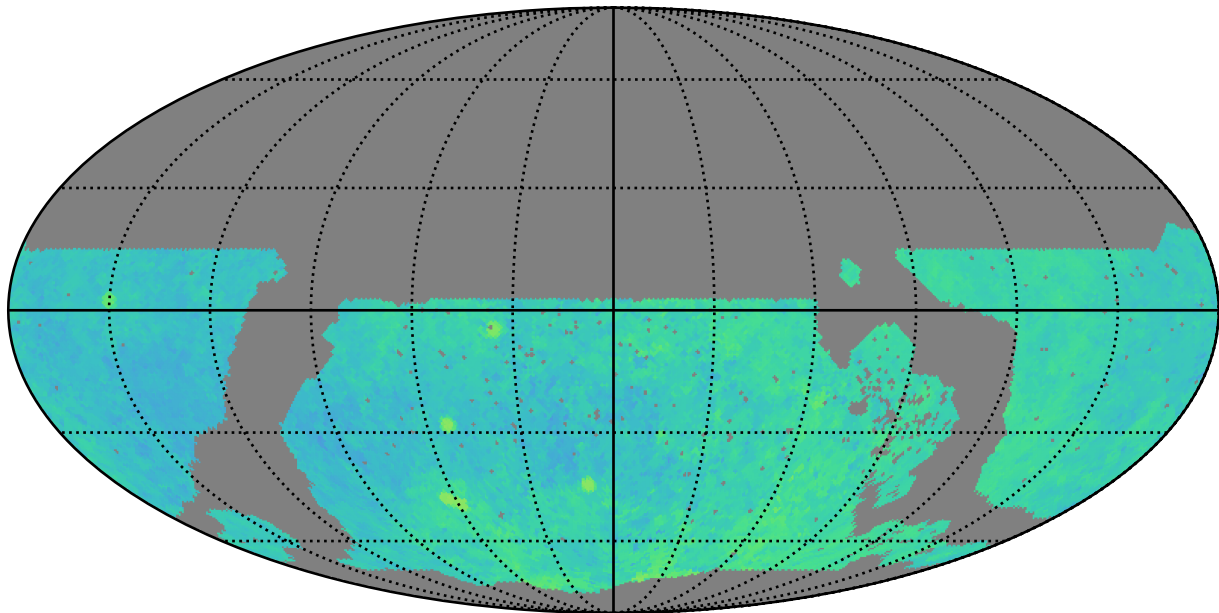
noroll_mjdp120_v3.4_10yrs WFD i band: Median Season Length
