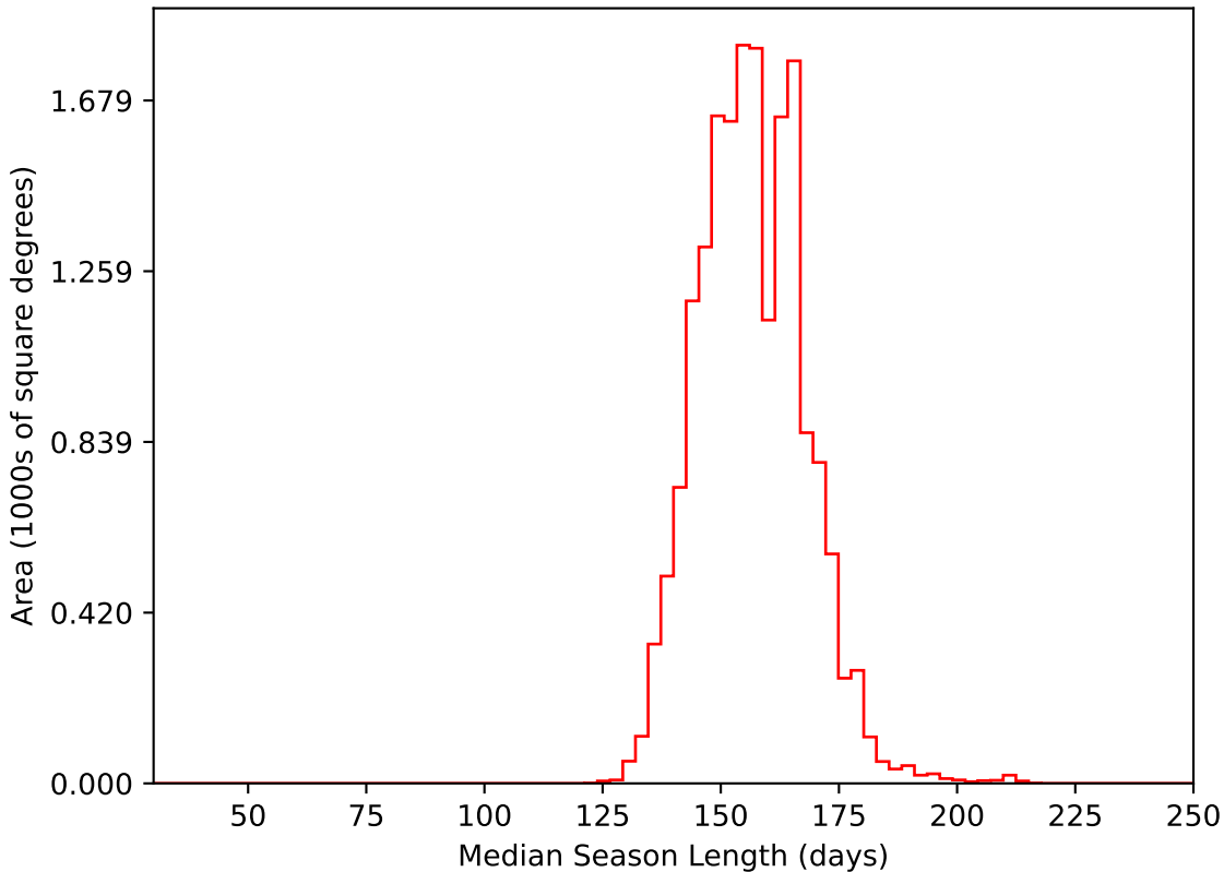
noroll_mjdp120_v3.4_10yrs WFD i band: Median Season Length
